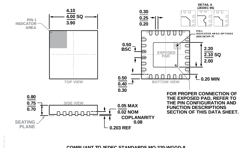
Figure 45. 24-Lead Lead Frame Chip Scale Package [LFCSP] 4 mm × 4 mm Body and 0.75 mm Package Height (CP-24-10)
