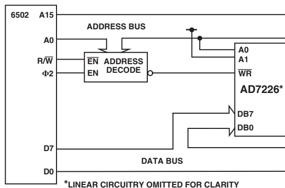
Figure 20. AD7226 to 6502 Interface
