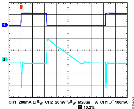
Figure 42. Output Transient Response, V_{OUT} = 5\text{ V} , C_{OUT} = 2.2\ \mu\text{F} , CH1 Load Current, CH2 V_{OUT}
