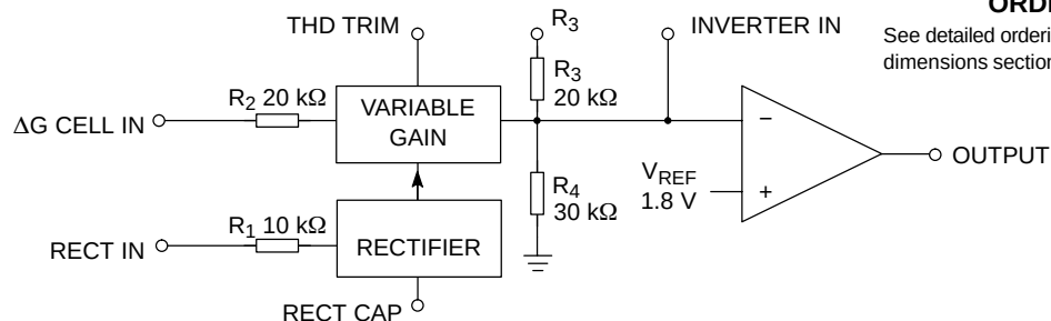
Figure 1. Block Diagram
