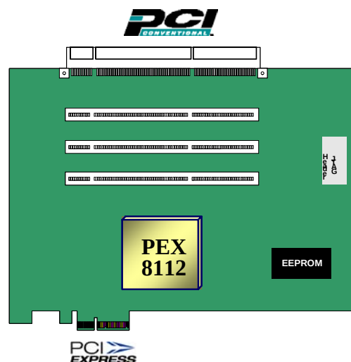
Figure 5. Forward Bridge RDK
