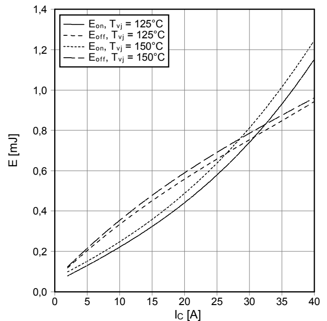
Schaltverluste IGBT-Wechselr. (typisch) switching losses IGBT-inverter (typical) E_{on} = f(I_C), E_{off} = f(I_C) V_{GE} = \pm 15\text{ V}, R_{Gon} = 18\ \Omega, R_{Goff} = 18\ \Omega, V_{CE} = 300\text{ V}
