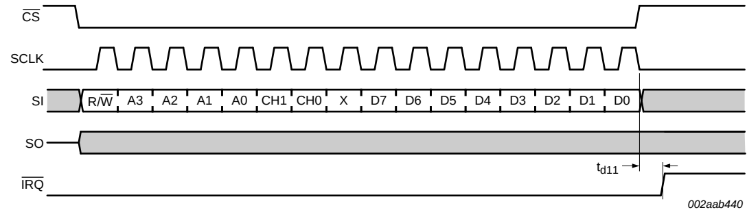
Fig 38. SPI write THR to clear TX INT
