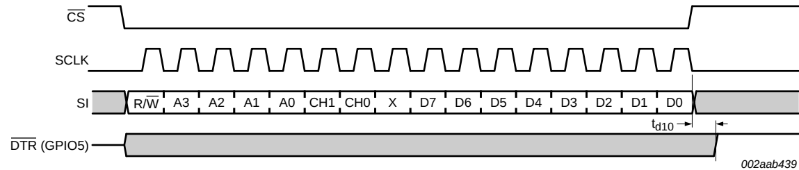
Fig 37. SPI write MCR to DTR output switch (SC16IS750 and SC16IS760 only)
