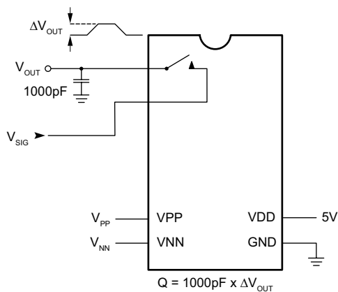
Charge Injection
