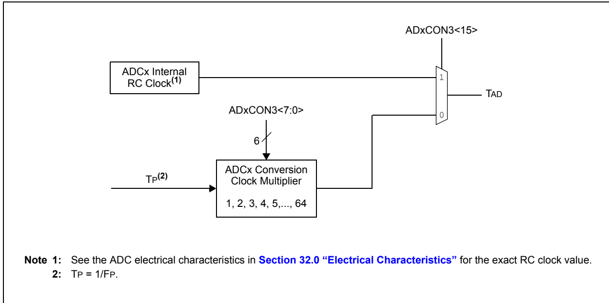
FIGURE 23-2: ADCx CONVERSION CLOCK PERIOD BLOCK DIAGRAM
