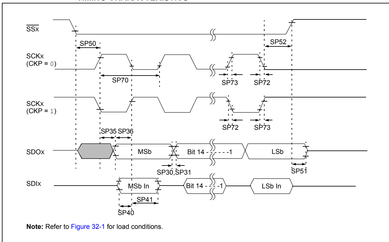
FIGURE 32-22: SPI1, SPI3 AND SPI4 SLAVE MODE (FULL-DUPLEX, CKE = 0, CKP = 0, SMP = 0) TIMING CHARACTERISTICS
