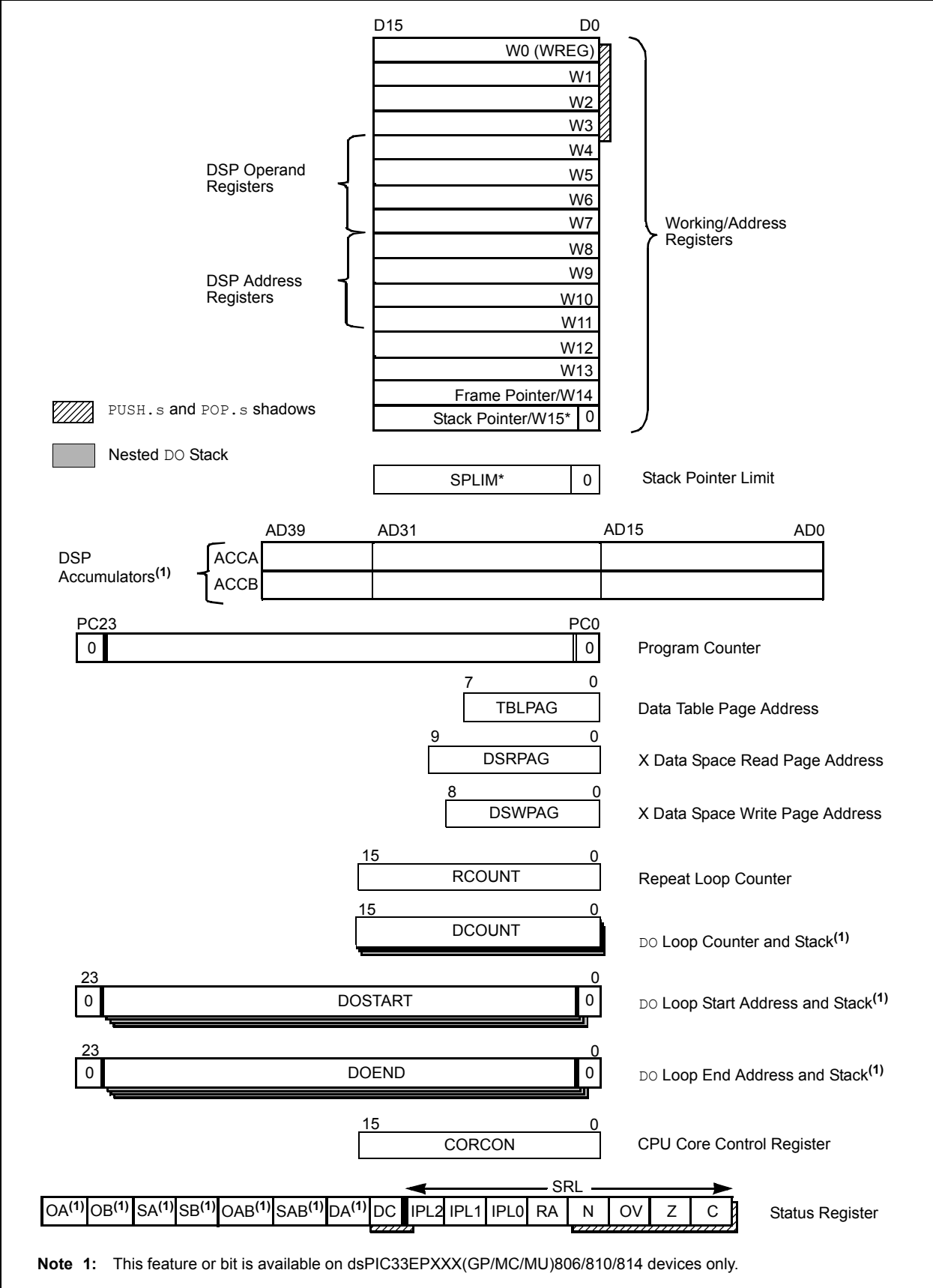
FIGURE 3-2: PROGRAMMER'S MODEL
