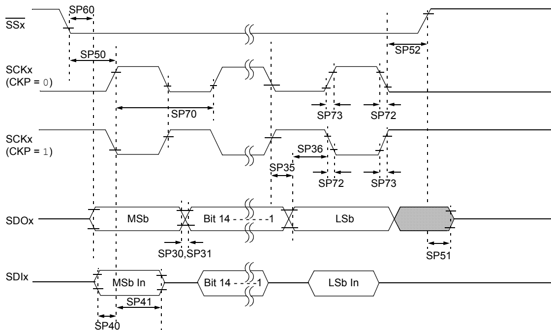
FIGURE 32-27: SPI2 SLAVE MODE (FULL-DUPLEX, CKE = 1, CKP = 0, SMP = 0) TIMING CHARACTERISTICS
