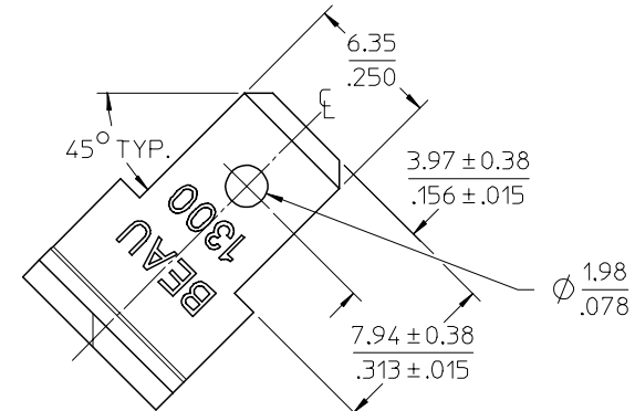
VIEW Z-Z
