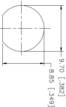
RECOMMENDED MOUNTING HOLE DIMENSIONS
