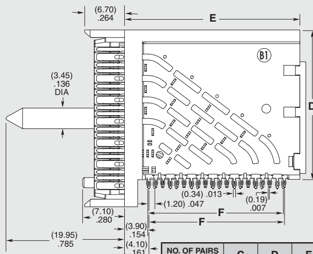
EBTM-6-12-2.0-S-RA-1-R-A SHOWN
