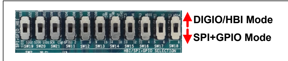
FIGURE 2-4: SW11-SW21 DIGIO/HBI/SPI+GPIO MODE SELECTION
