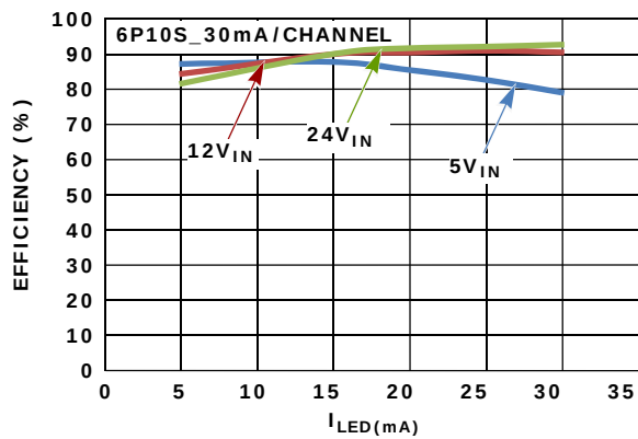
FIGURE 4. EFFICIENCY vs up to 30mA LED CURRENT (100 % LED DUTY CYCLE) vs V_{IN}
