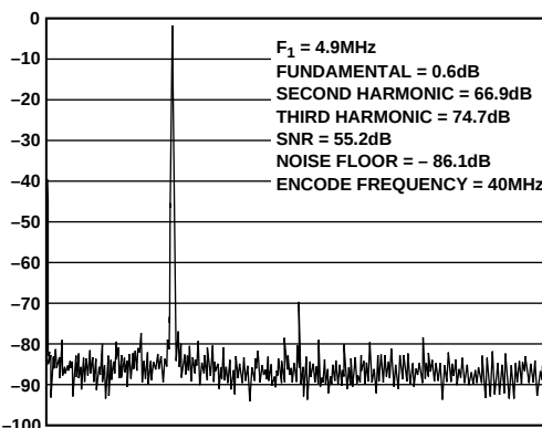
Figure 10. FFT Output of Circuit in Figure 9
