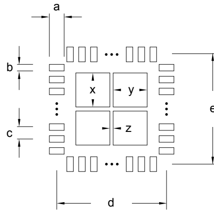
Figure 10.4. QFN64 PCB Stencil Design
