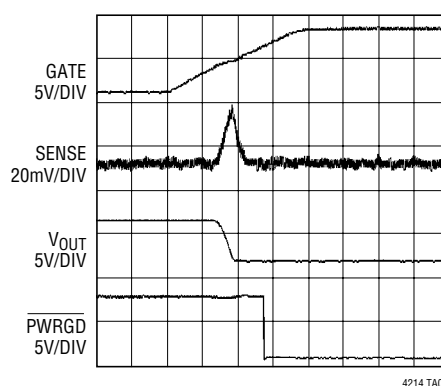
Start-Up Behavior
