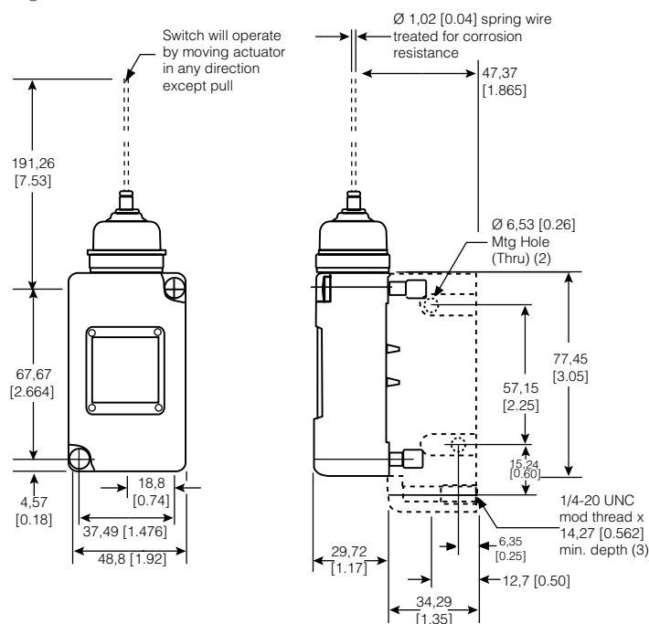
Figure 22. 208LS125 Dimensions
