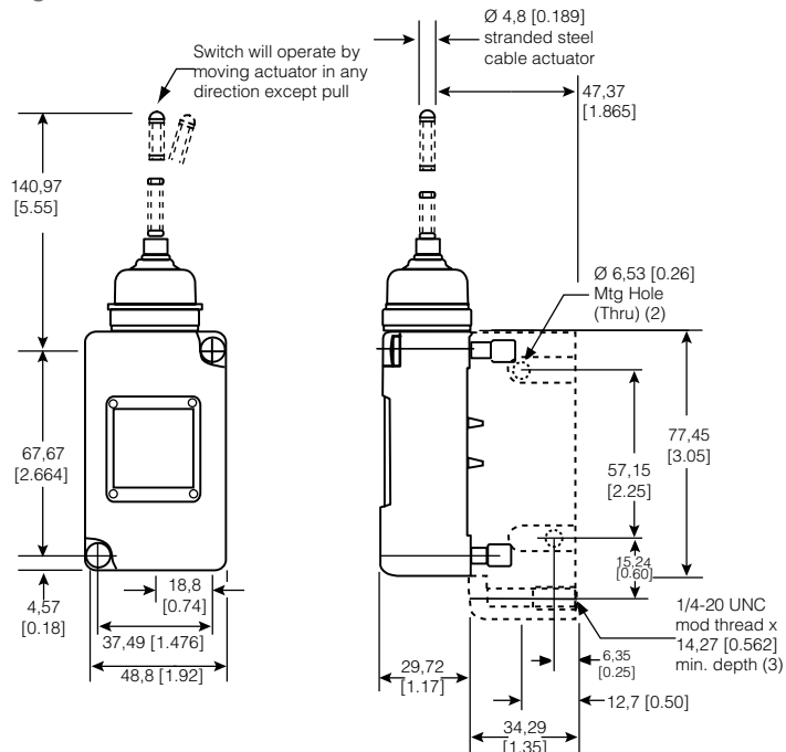
Figure 20. 208LS1 Dimensions
