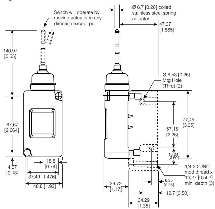
Figure 23. 208LS152 Dimensions
