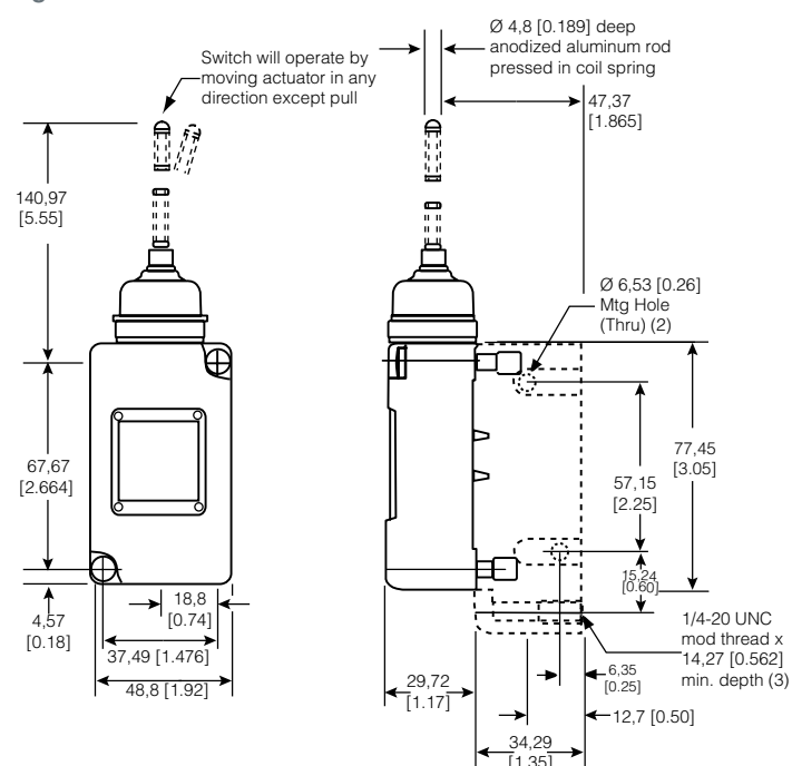
Figure 21. 208LS3 Dimensions
