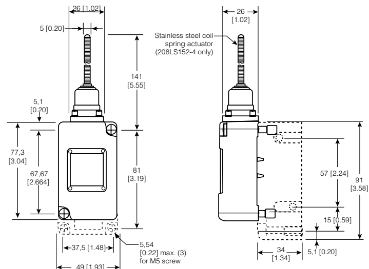
Figure 39. 208LS1-4 Dimensions
