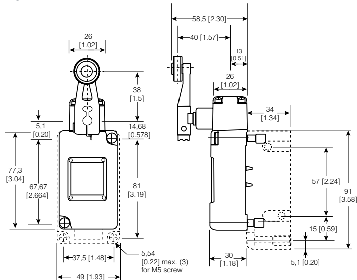
Figure 36. 202LS1-4 Dimensions
