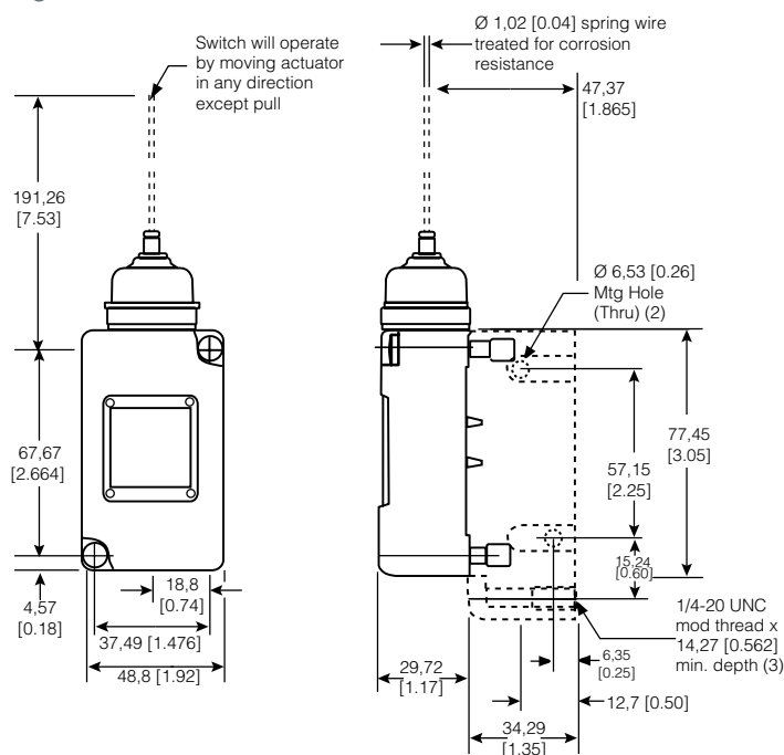
Figure 22. 208LS125 Dimensions
