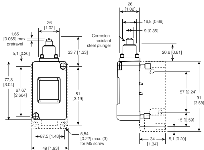
Figure 37. 204LS1-4 Dimensions
