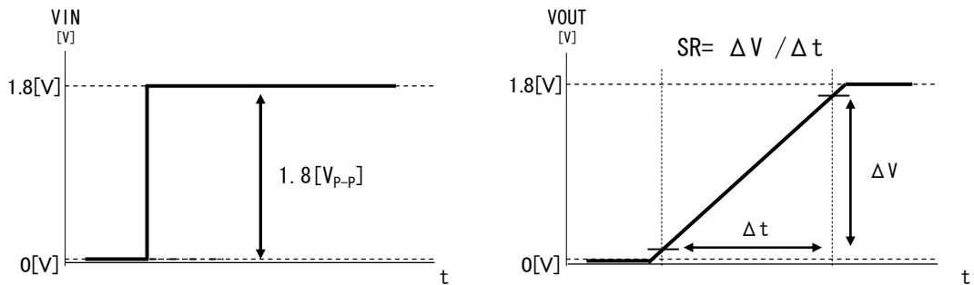
Fig.97 Slew rate input output wave (Ground Sense BU7411 family, BU7421 family)
