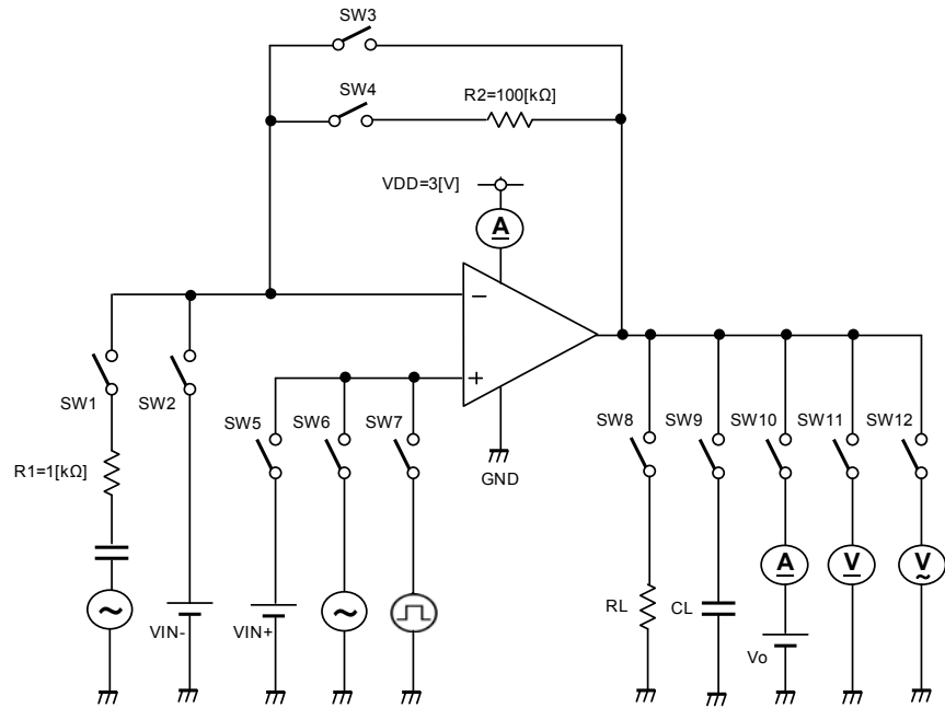
Fig.95 Test circuit2
