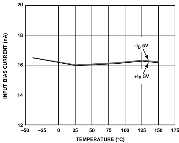
Figure 11. Input Bias Current at V_{POS} , V_{NEG} vs. Temperature, V_{SY} = 5\text{ V} , 2.7\text{ V}
