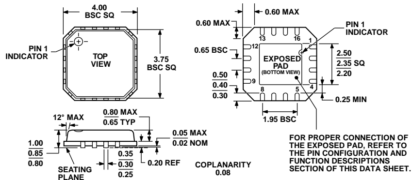
Figure 49. 16-Lead Lead Frame Chip Scale Package [LFCSP_VQ] 4 mm × 4 mm Body, Very Thin Quad (CP-16-10) Dimensions shown in millimeters
