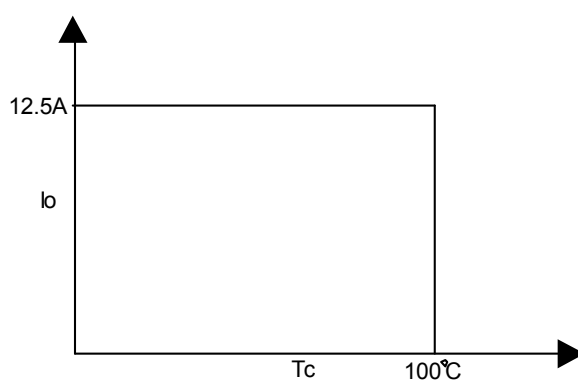
Figure 19 Output power derating, 24V in
