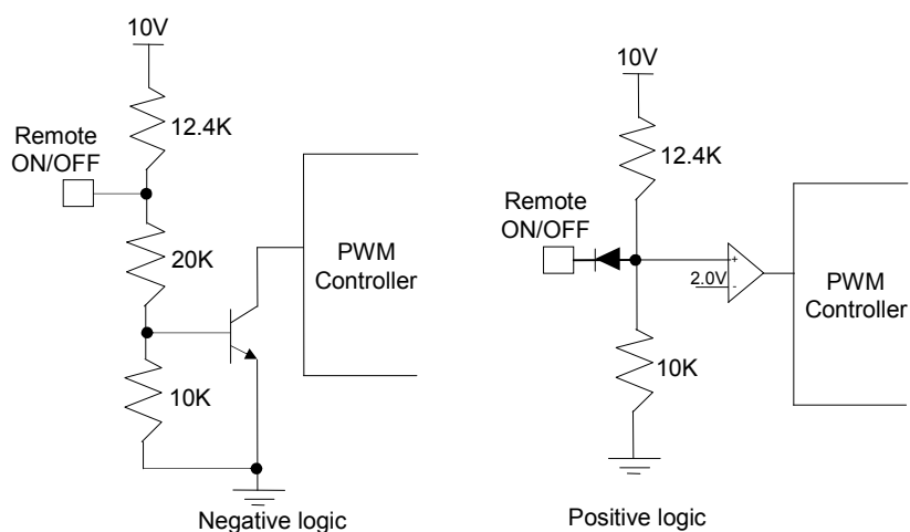
Figure 11 Remote ON/OFF internal diagram
