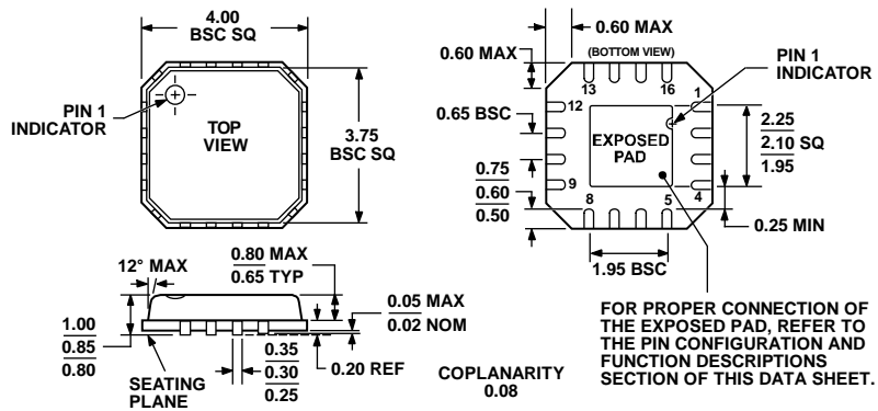
Figure 39.16-Lead Lead Frame Chip Scale Package [LFCSP_VQ] 4 mm x 4 mm Body, Very Thin Quad (CP-16-4) Dimensions shown in millimeters
