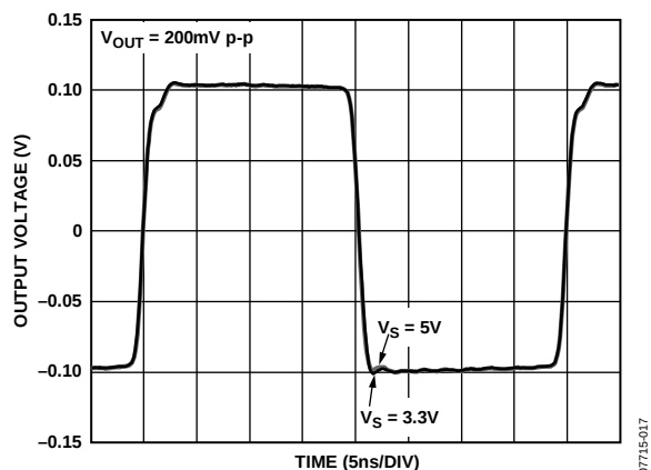
Figure 17. Small Signal Transient Response vs. Supply Voltage, C_L = 4 \text{ pF}
