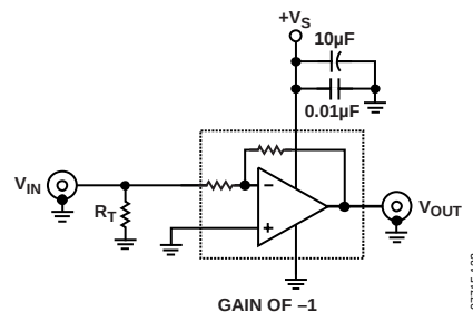
Figure 34. Inverting Configuration ( G = -1 )
