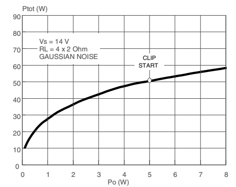
Figure 13. Power Dissipation vs. Average Output Power (Audio Program Simulation, 2\Omega )
