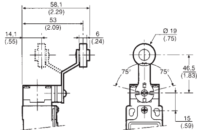
Offset Side Rotary Roller Lever A5A Plastic Roller A5B Metal Roller Head
