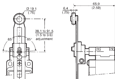
Side Rotary Adjustable Lever A2A Plastic Roller A2B Metal Roller
