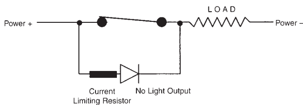
Typical Wiring Arrangement 2
