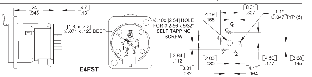
FEMALE CONNECTOR GROUND TO PIN #1 OPTION "G1"
