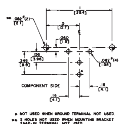
RECOMMENDED PC BOARD LAYOUT (STRAIGHT)
