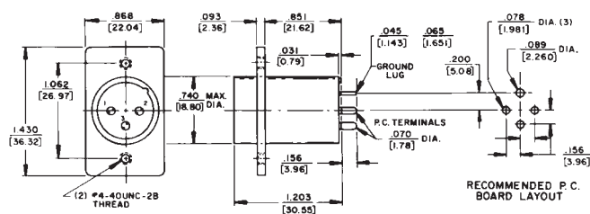
(Component Side)
