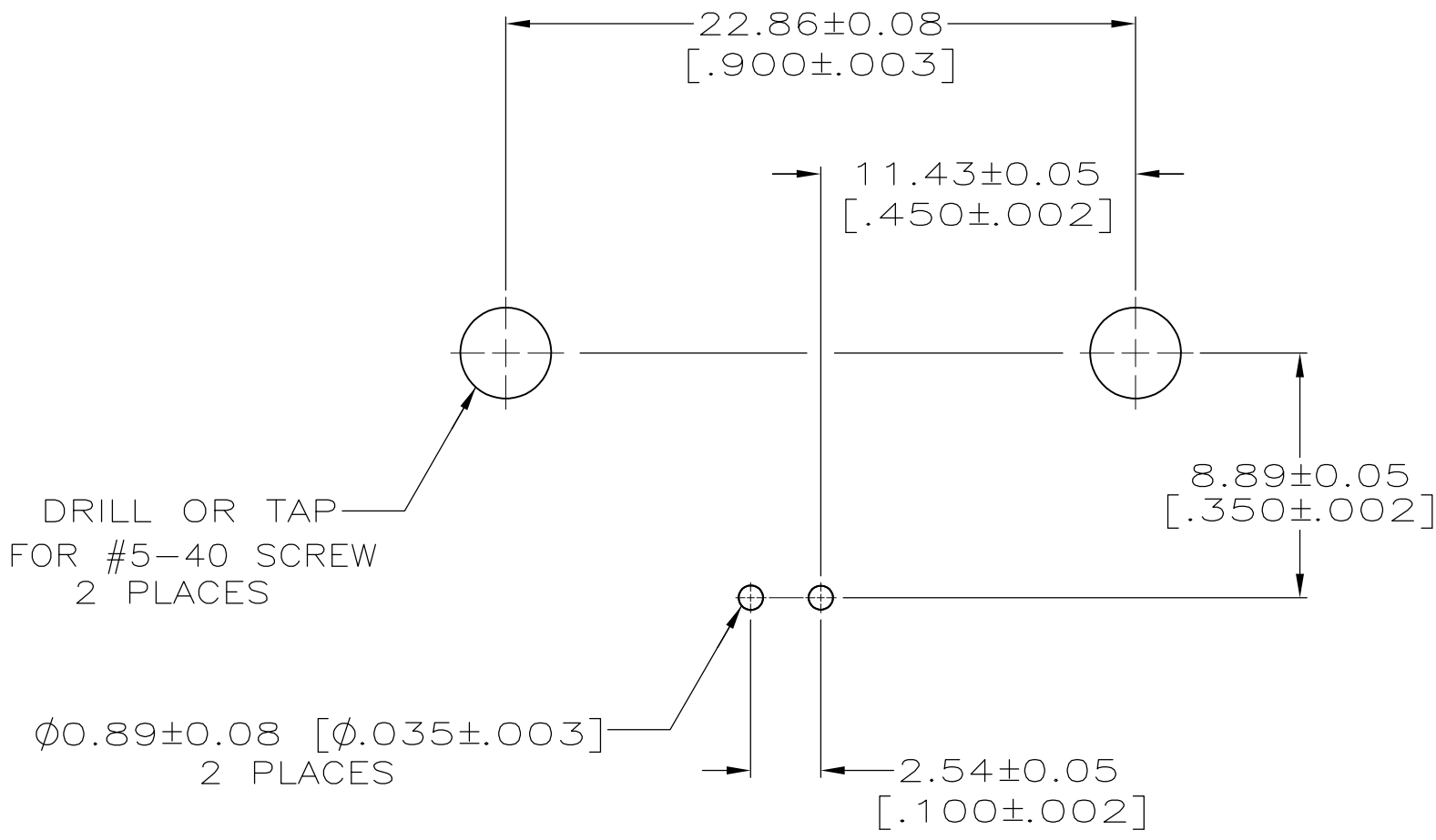
PCB CONFIGURATION
