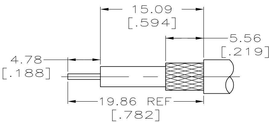
RECOMMENDED STRIP LENGTH SCALE: 3:1
