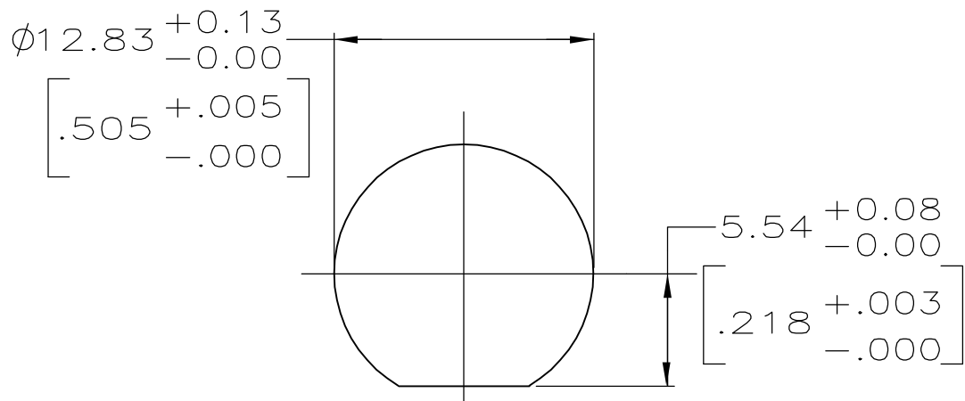
RECOMMENDED PANEL CUTOUT SCALE: 3:1
