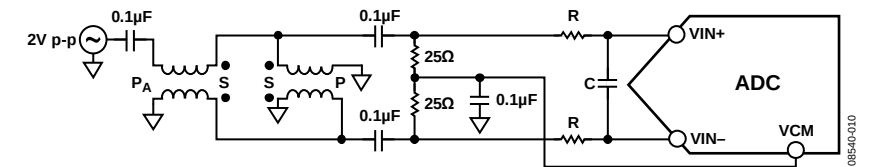
Figure 40. Differential Double Balun Input Configuration
