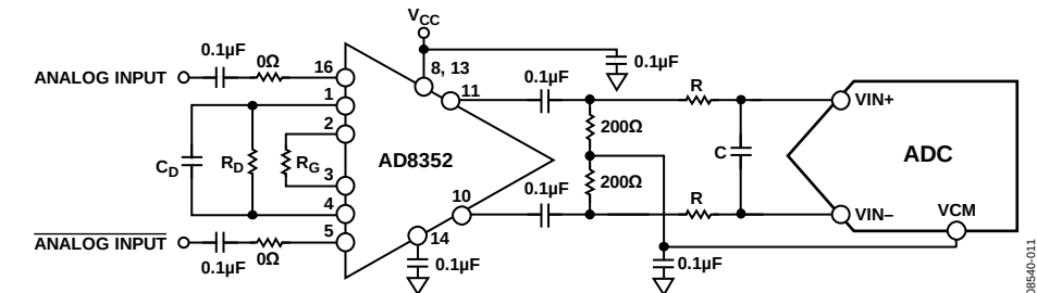
Figure 41. Differential Input Configuration Using the AD8352
