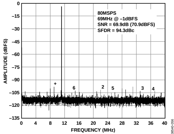
Figure 5. AD9629-80 Single-Tone FFT with f_{IN} = 69 MHz
