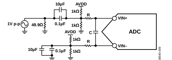
Figure 39. Single-Ended Input Configuration
