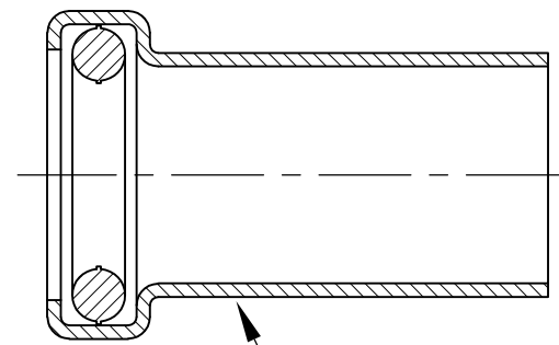
1 FERRULE
