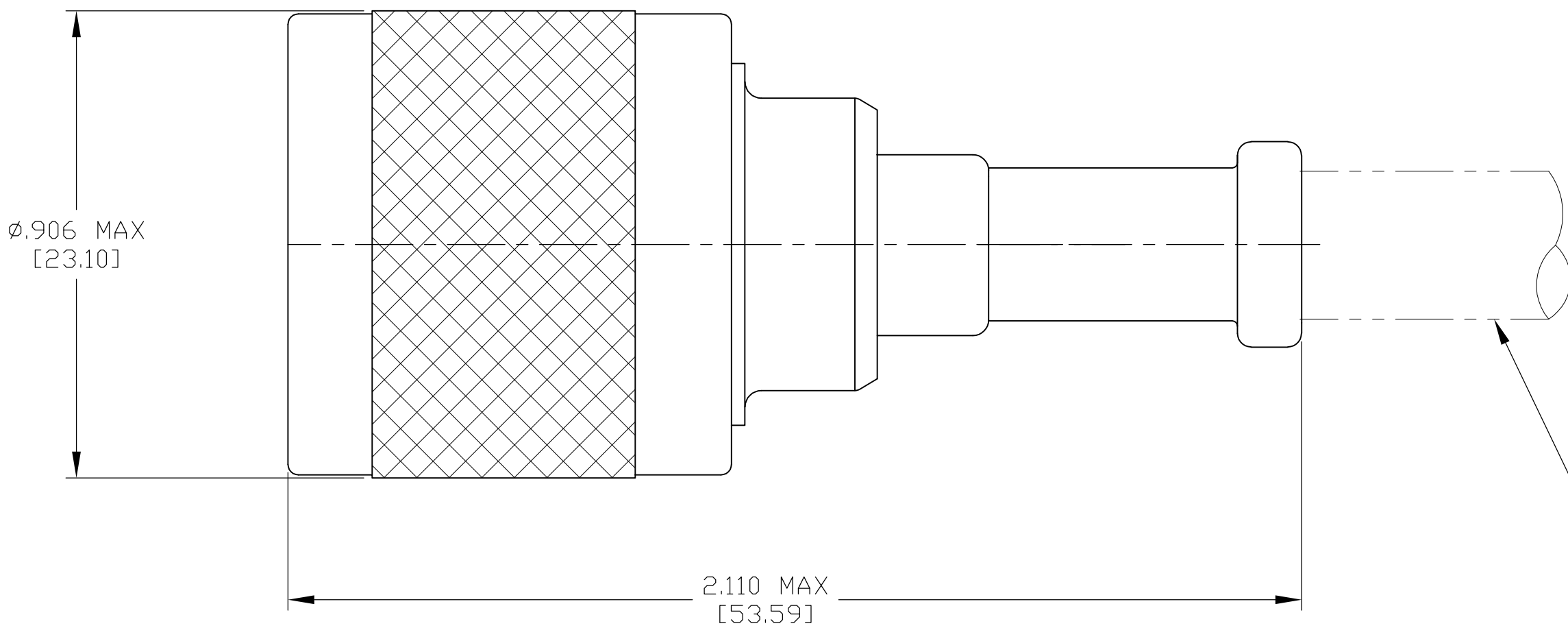
ASSEMBLED VIEW
