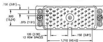
56 PIN PLUG
