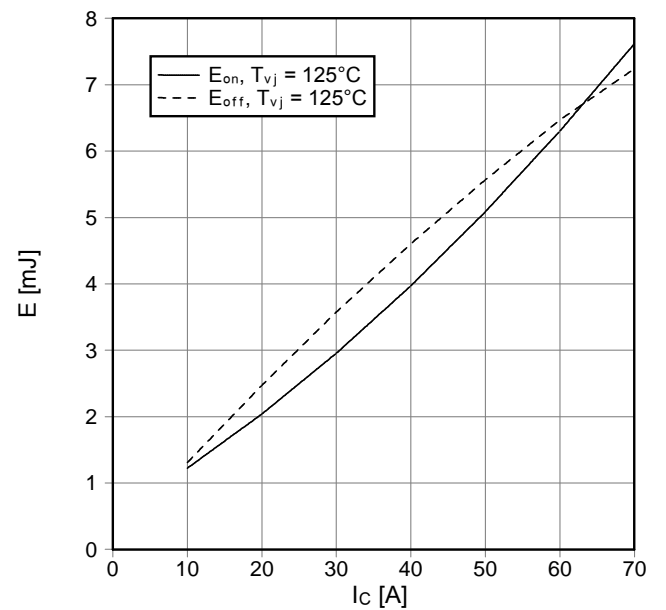
Schaltverluste IGBT-Wechselr. (typisch) switching losses IGBT-inverter (typical) E_{on} = f(I_C) , E_{off} = f(I_C) V_{GE} = \pm 15\text{ V} , R_{Gon} = 27\ \Omega , R_{Goff} = 27\ \Omega , V_{CE} = 600\text{ V}
