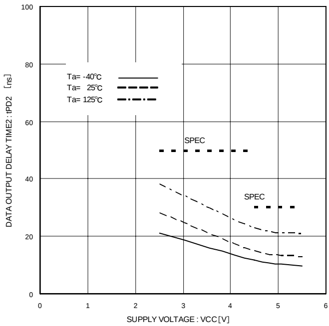
Figure 26. Data Output Delay Time t_{PD2} ( C_L=30\text{pF} )
