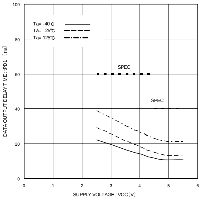
Figure 25. Data Output Delay Time t_{PD1} ( C_L=100\text{pF} )
