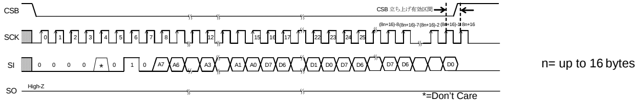
Figure 39. N Byte page write command
