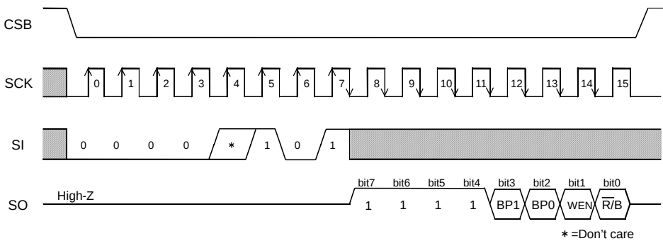
Figure 42. Status register read command
