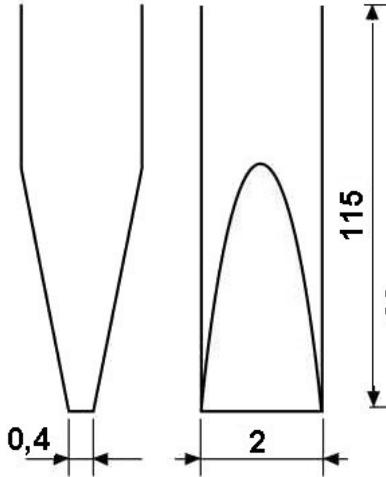
Dimensioned drawing
