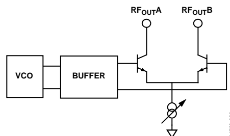
Figure 20. Output Stage ADF4360-8
