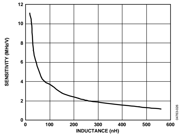
FIXED FREQUENCY LO
