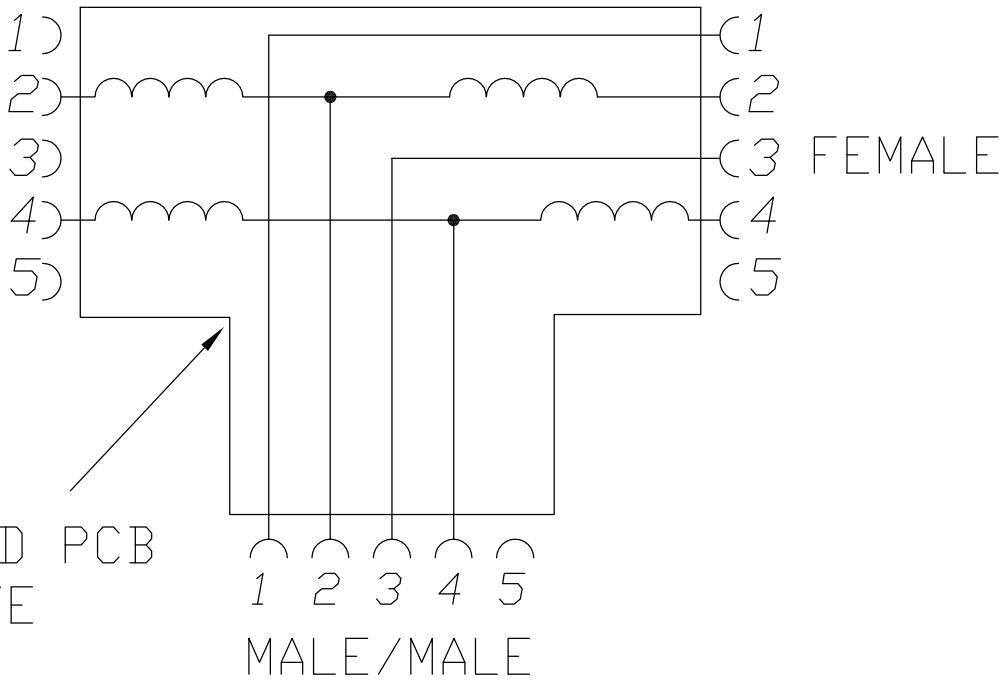
WIRING DIAGRAM
