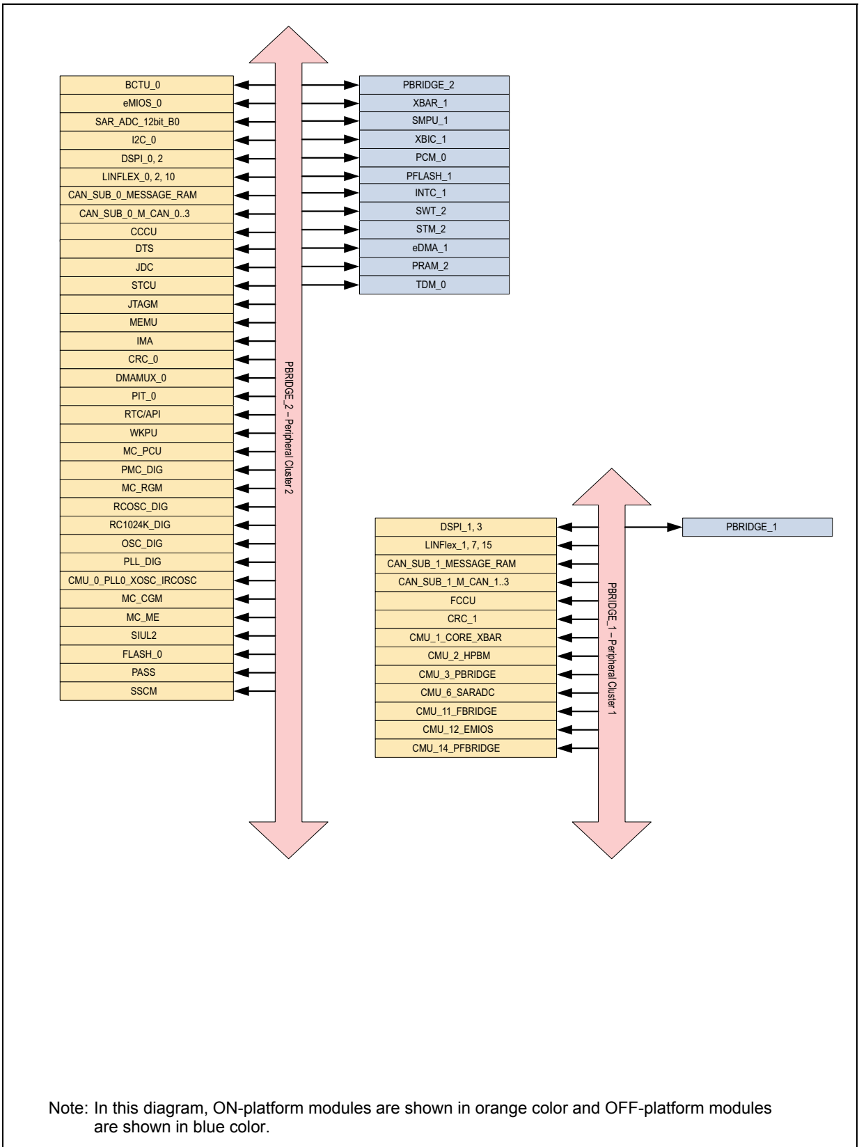
Figure 2. Periphery allocation
