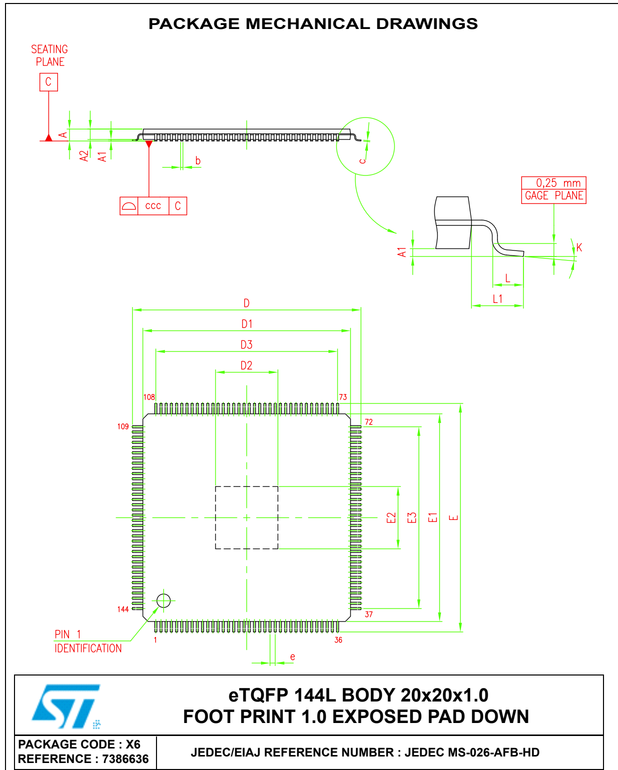
Figure 32. eTQFP144 package outline
