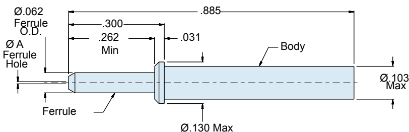
181-057 Pin Terminus
