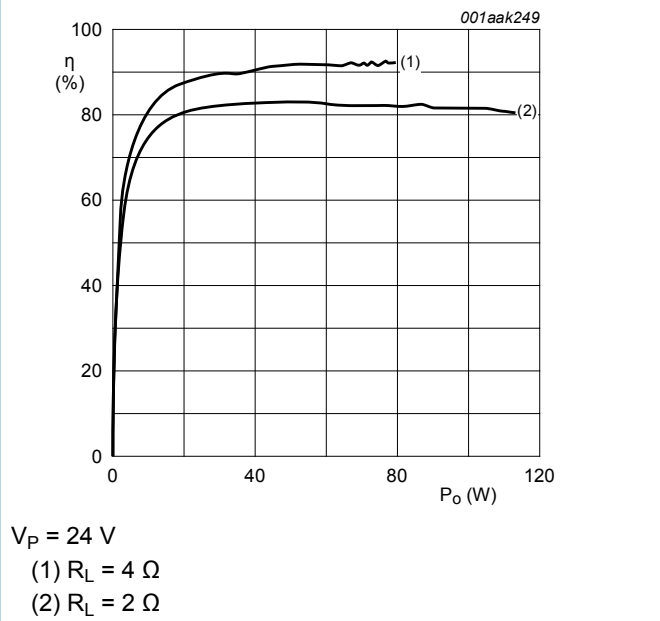
Figure 45. Efficiency as a function of total output power with both channels driven; V_P = 24 V
