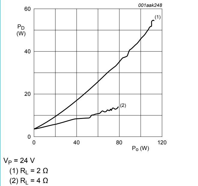
Figure 44. Power dissipation as a function of total output power with both channels driven; V_P = 24 V
