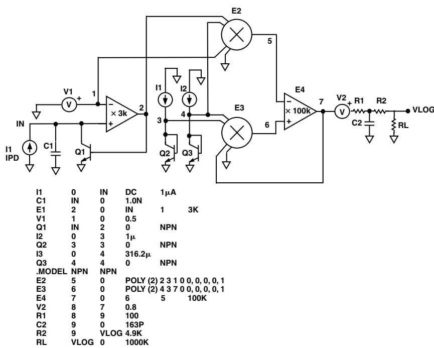
Figure 12. Basic Macromodel
